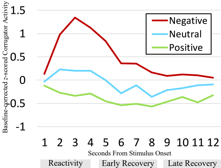
Figure 1. Time-course for baseline-corrected z-scored corrugator activity by image valence condition. For each time-window (reactivity, early recovery, and late recovery), mean corrugator activity was larger for negative than neutral and larger for neutral than positive.
