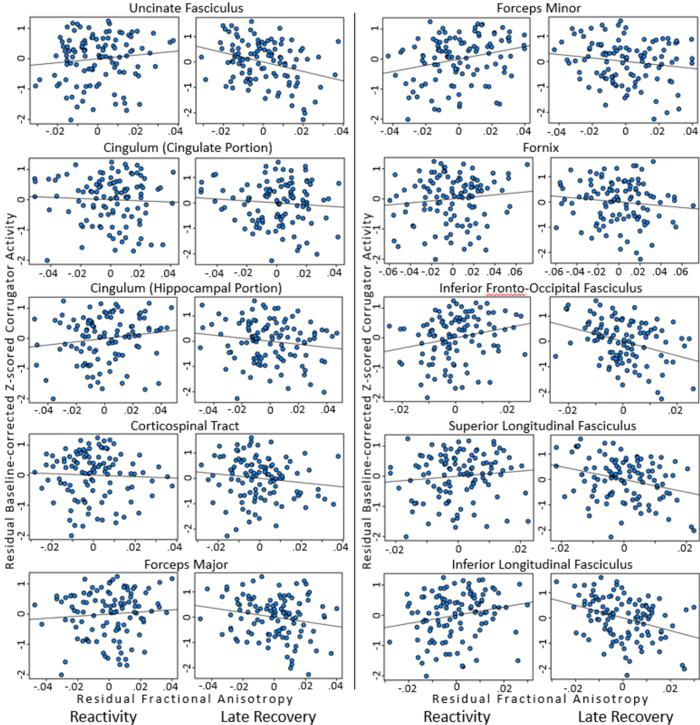
Figure 2. Partial plots depicting relationship between fractional anisotropy (FA) and mean baseline-corrected z-scored corrugator activity in response to negative images for reactivity (left), and late recovery (right) time windows while controlling for global FA. Late corrugator activity was significantly related to FA in the uncinate, inferior longitudinal, inferior fronto-occipital, and superior longitudinal fasciculi. Mean FA was not related to corrugator reactivity for any tract.
